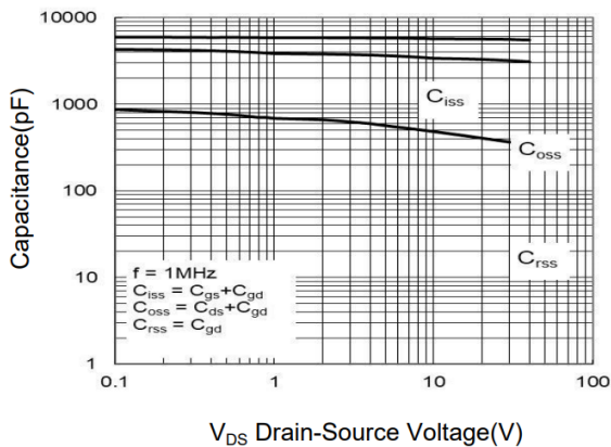
Figure 5. Capacitance Characteristics
