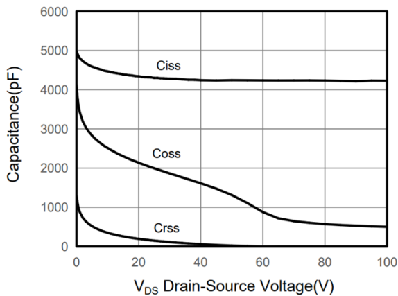
Figure 5. Capacitance Characteristics
