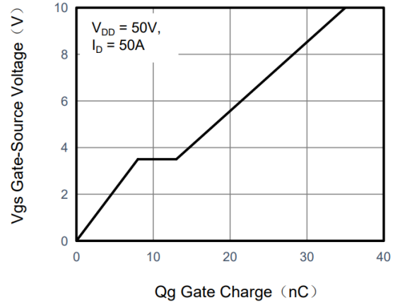
Figure 4. Gate Charge
