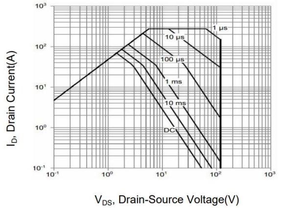
Figure 8. Safer Operation Area
