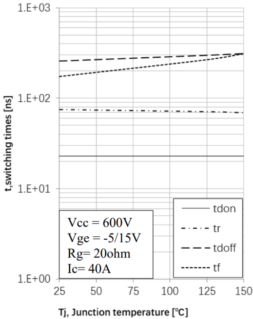
Figure 9. Typical Switching times as a function of junction temperature
