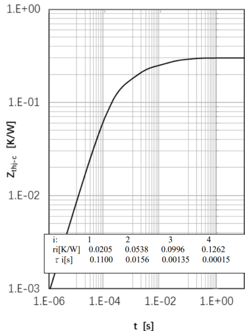
Figure 16. IGBT Transient Thermal Impedance
