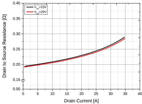
Figure 3. Drain to Source Resistance vs Drain Current
