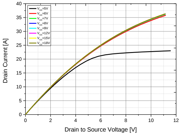
Figure 1. On-state characteristics
